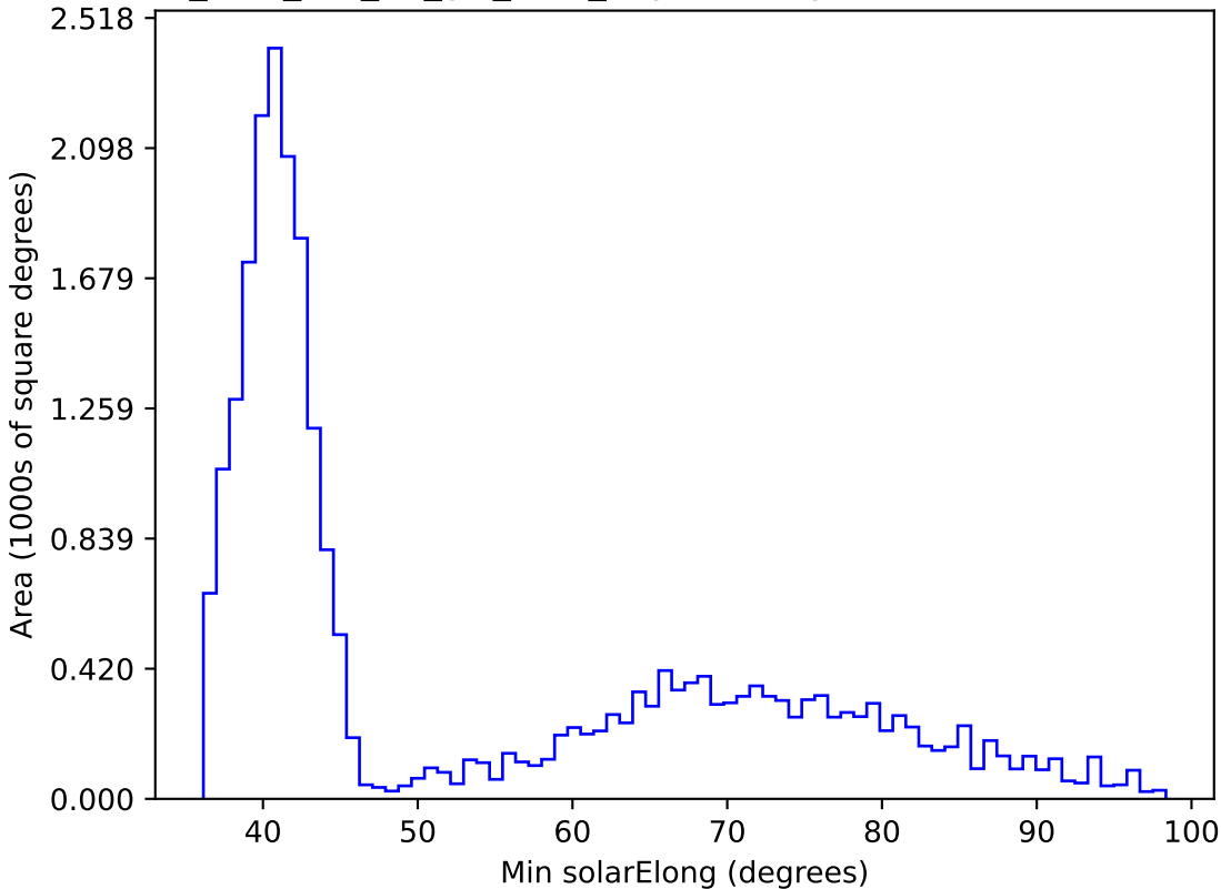
too_elab_r32_d3_giz_v3.4_10yrs All sky i band: Min solarElong
