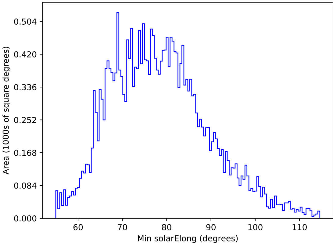
too_elab_r32_d3_giz_v3.4_10yrs All sky g band: Min solarElong
