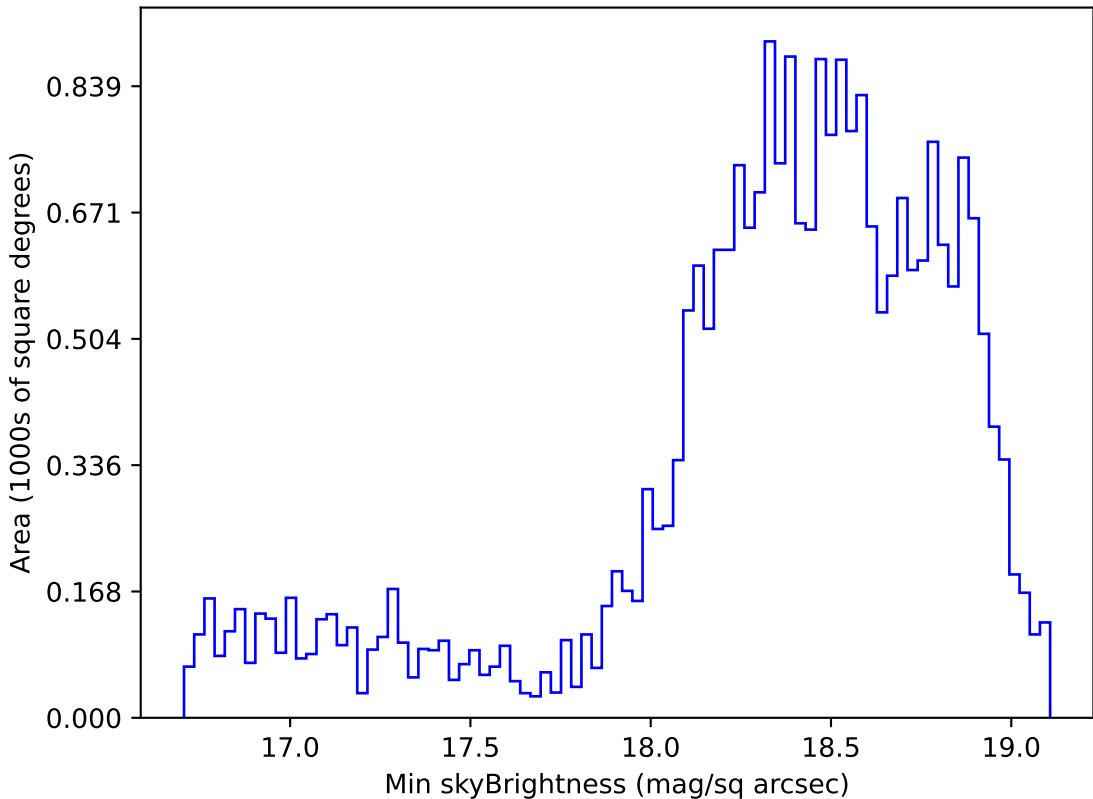
too_elab_r32_d3_giz_v3.4_10yrs Yr 1 z band: Min skyBrightness
