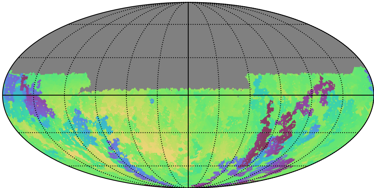
too_elab_r32_d3_giz_v3.4_10yrs Yr 1 u band: Min skyBrightness
