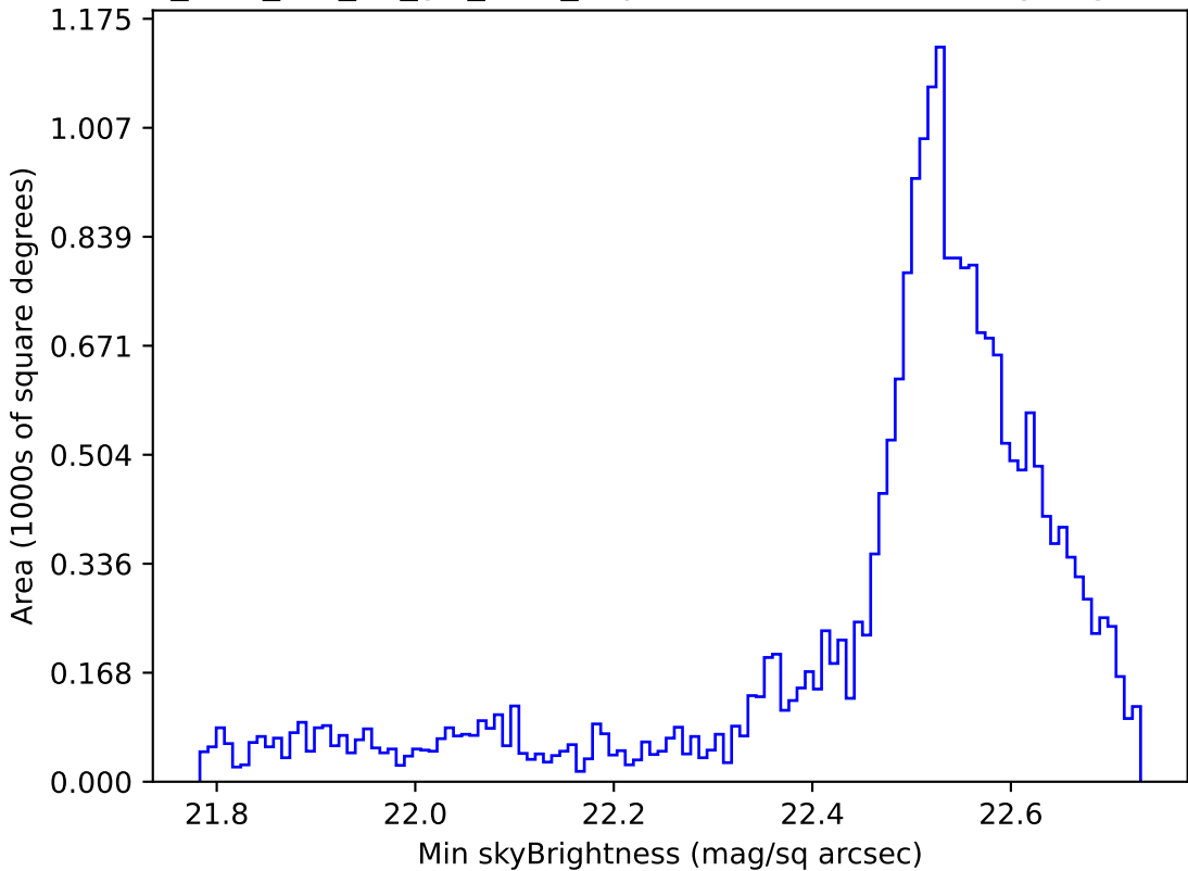
too_elab_r32_d3_giz_v3.4_10yrs Yr 1 u band: Min skyBrightness
