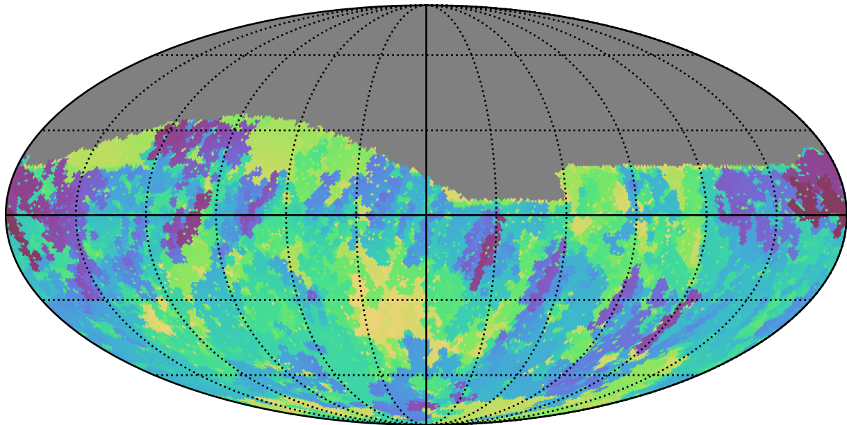
too_elab_r32_d3_giz_v3.4_10yrs Yr 1 r band: Min skyBrightness
