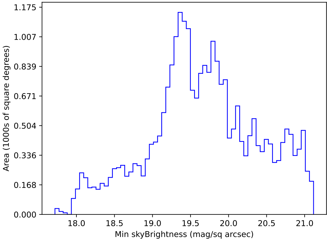
too_elab_r32_d3_giz_v3.4_10yrs Yr 1 r band: Min skyBrightness
