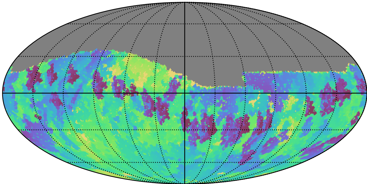
too_elab_r32_d3_giz_v3.4_10yrs Yr 1 i band: Min skyBrightness
