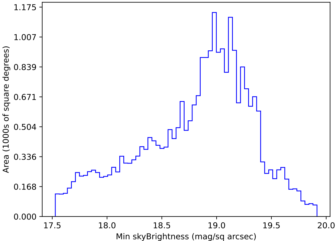
too_elab_r32_d3_giz_v3.4_10yrs Yr 1 i band: Min skyBrightness
