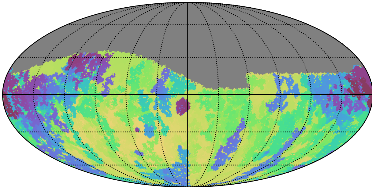
too_elab_r32_d3_giz_v3.4_10yrs Yr 1 g band: Min skyBrightness
