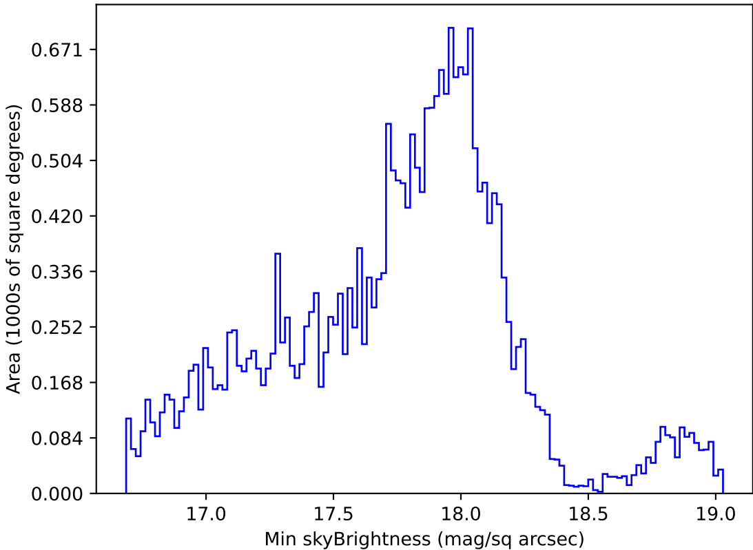
too_elab_r32_d3_giz_v3.4_10yrs Yr 1 all bands: Min skyBrightness
