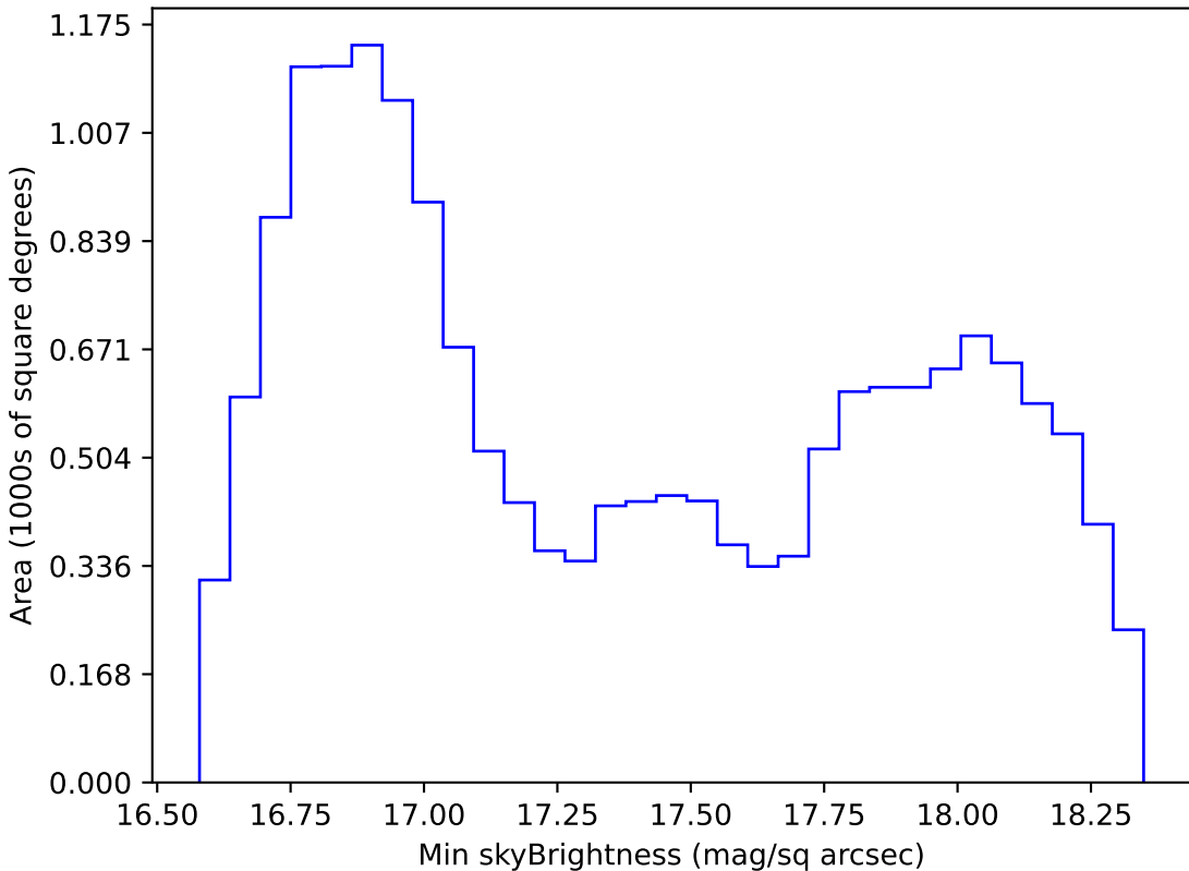
too_elab_r32_d3_giz_v3.4_10yrs WFD z band: Min skyBrightness
