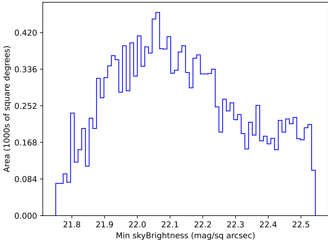
too_elab_r32_d3_giz_v3.4_10yrs WFD u band: Min skyBrightness
