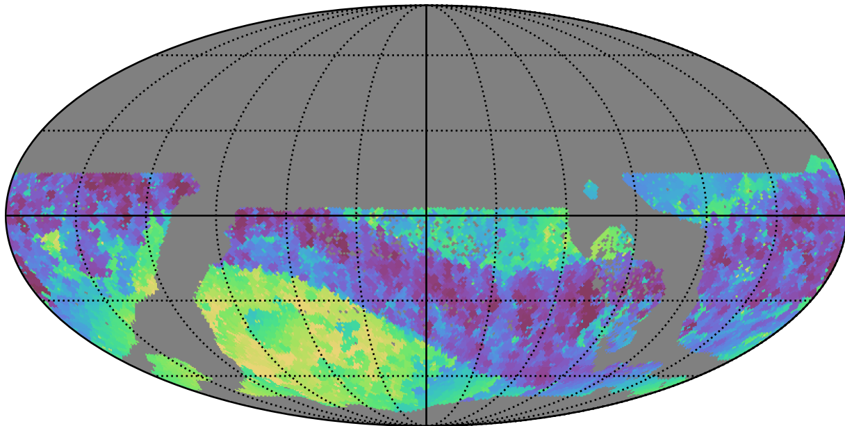
too_elab_r32_d3_giz_v3.4_10yrs WFD i band: Min skyBrightness
