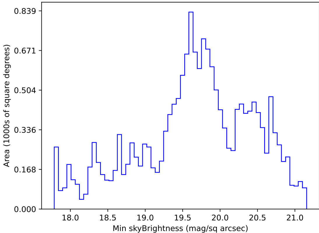
too_elab_r32_d3_giz_v3.4_10yrs WFD g band: Min skyBrightness
