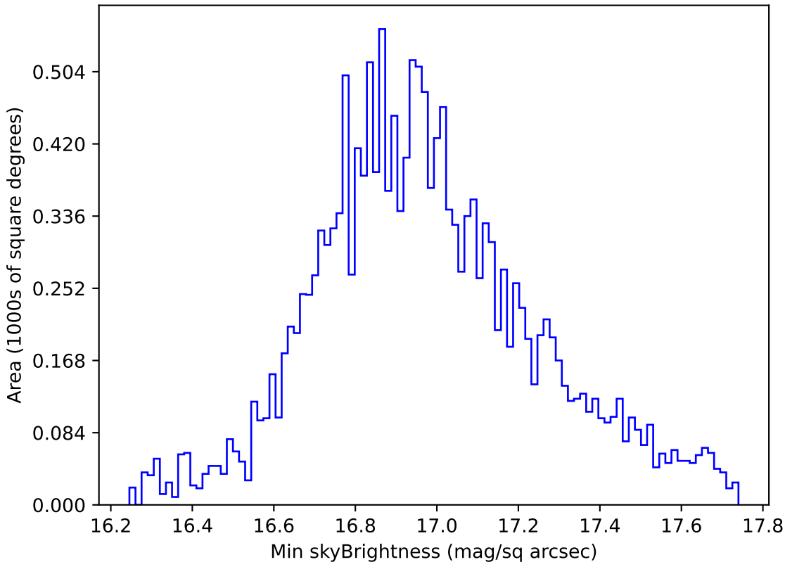
too_elab_r32_d3_giz_v3.4_10yrs WFD all bands: Min skyBrightness
