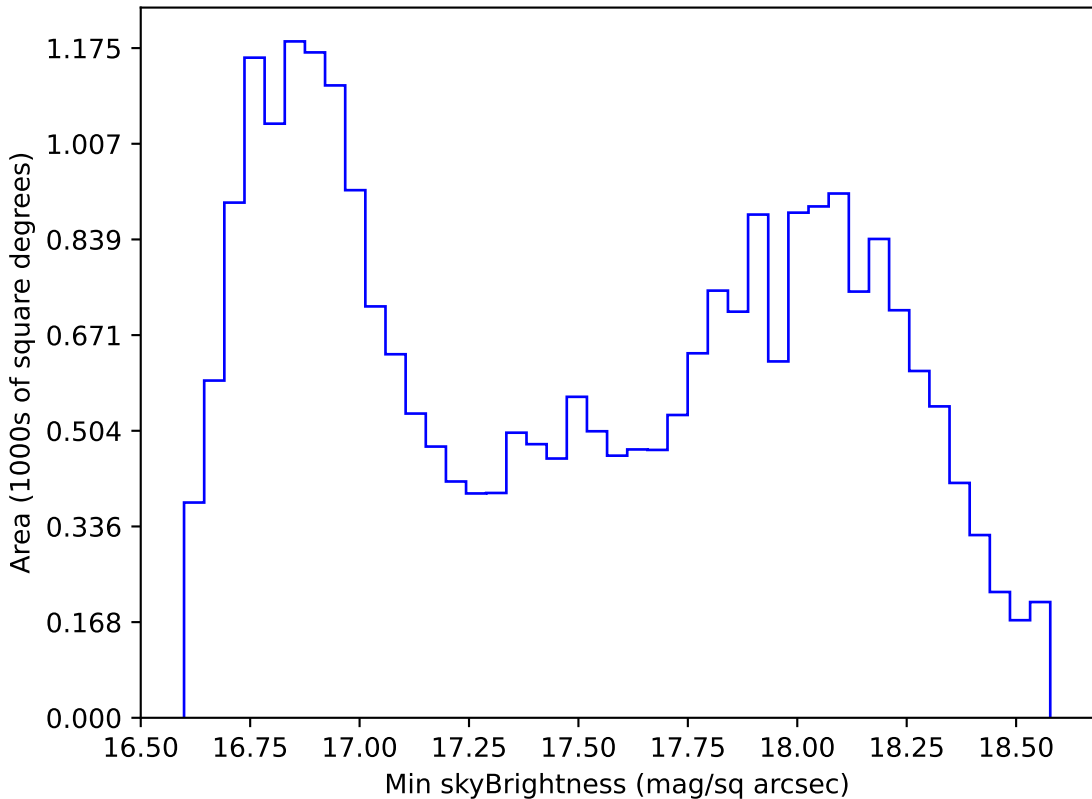
too_elab_r32_d3_giz_v3.4_10yrs All sky z band: Min skyBrightness
