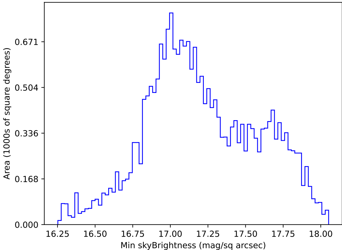
too_elab_r32_d3_giz_v3.4_10yrs All sky y band: Min skyBrightness
