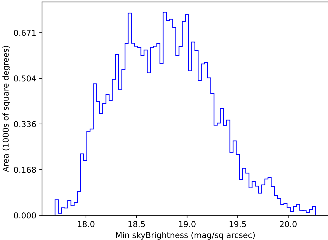
too_elab_r32_d3_giz_v3.4_10yrs All sky r band: Min skyBrightness
