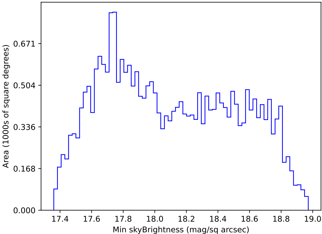
too_elab_r32_d3_giz_v3.4_10yrs All sky i band: Min skyBrightness
