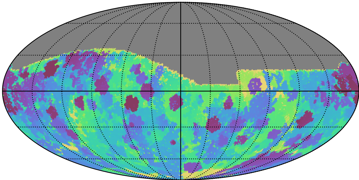
too_elab_r32_d3_giz_v3.4_10yrs All sky g band: Min skyBrightness
