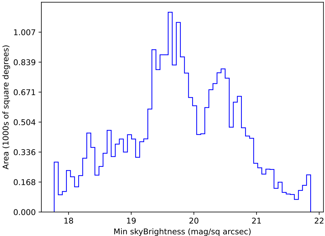
too_elab_r32_d3_giz_v3.4_10yrs All sky g band: Min skyBrightness
