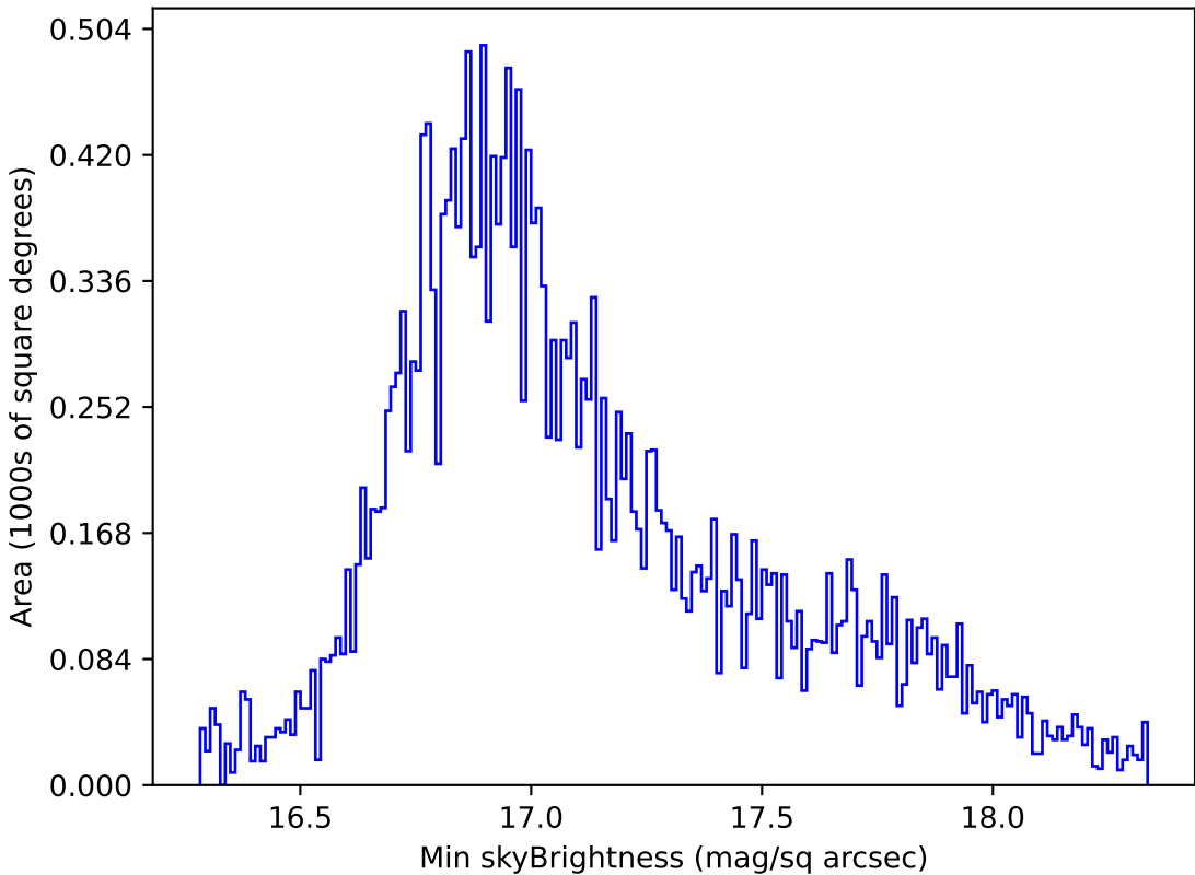
too_elab_r32_d3_giz_v3.4_10yrs All sky all bands: Min skyBrightness
