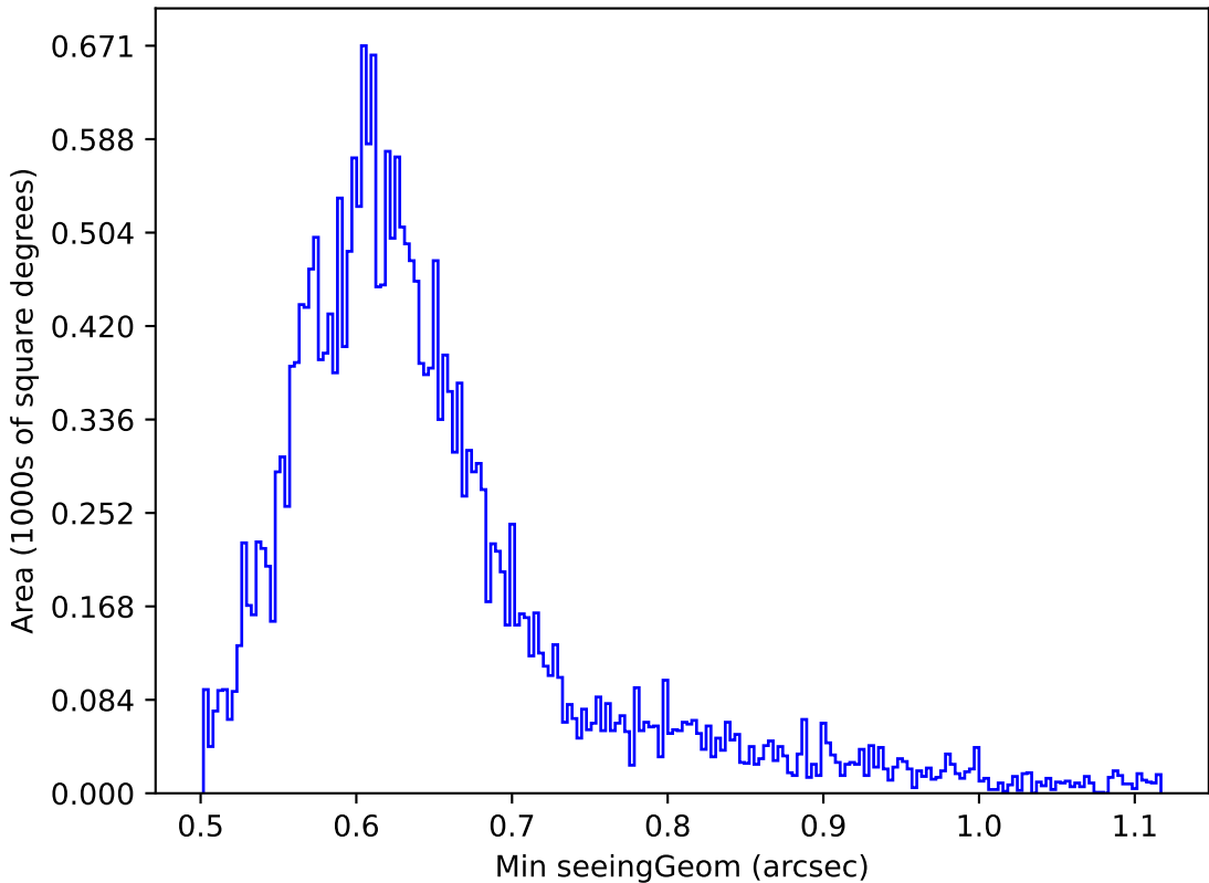
too_elab_r32_d3_giz_v3.4_10yrs Yr 1 z band: Min seeingGeom
