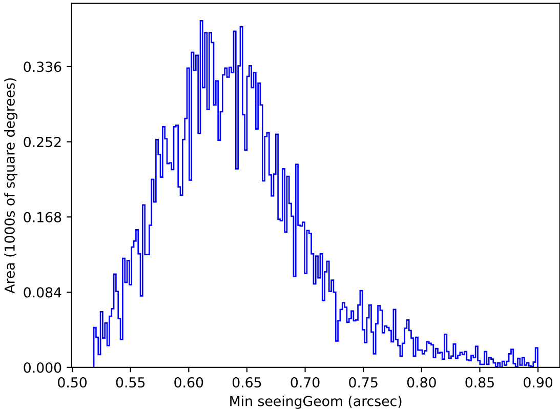
too_elab_r32_d3_giz_v3.4_10yrs Yr 1 y band: Min seeingGeom
