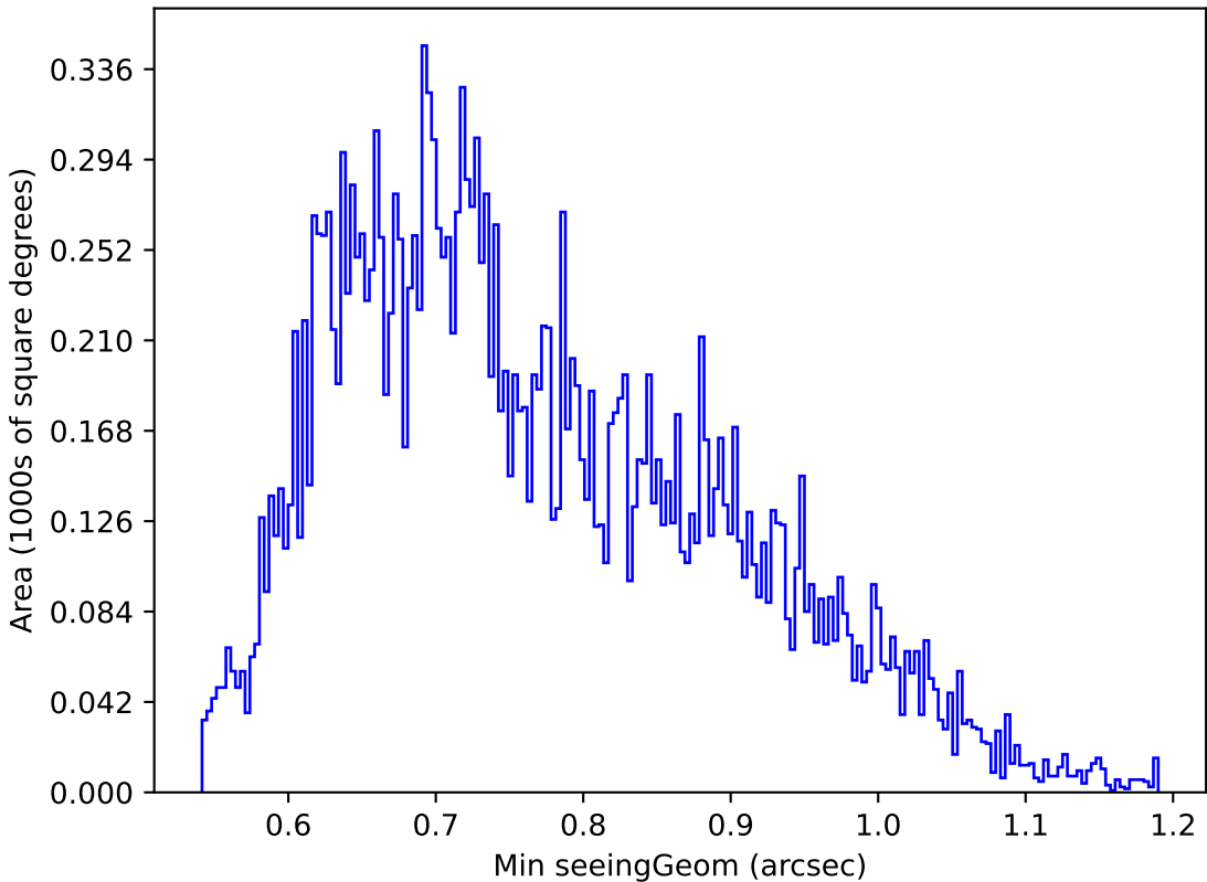
too_elab_r32_d3_giz_v3.4_10yrs Yr 1 u band: Min seeingGeom
