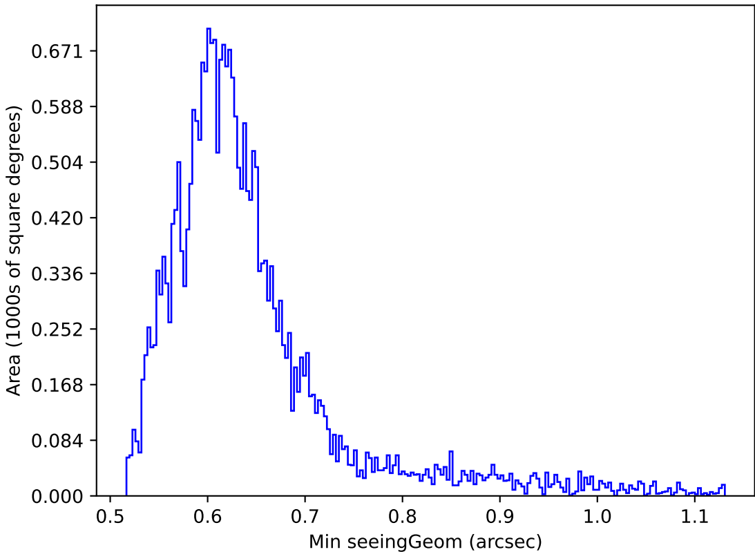
too_elab_r32_d3_giz_v3.4_10yrs Yr 1 r band: Min seeingGeom
