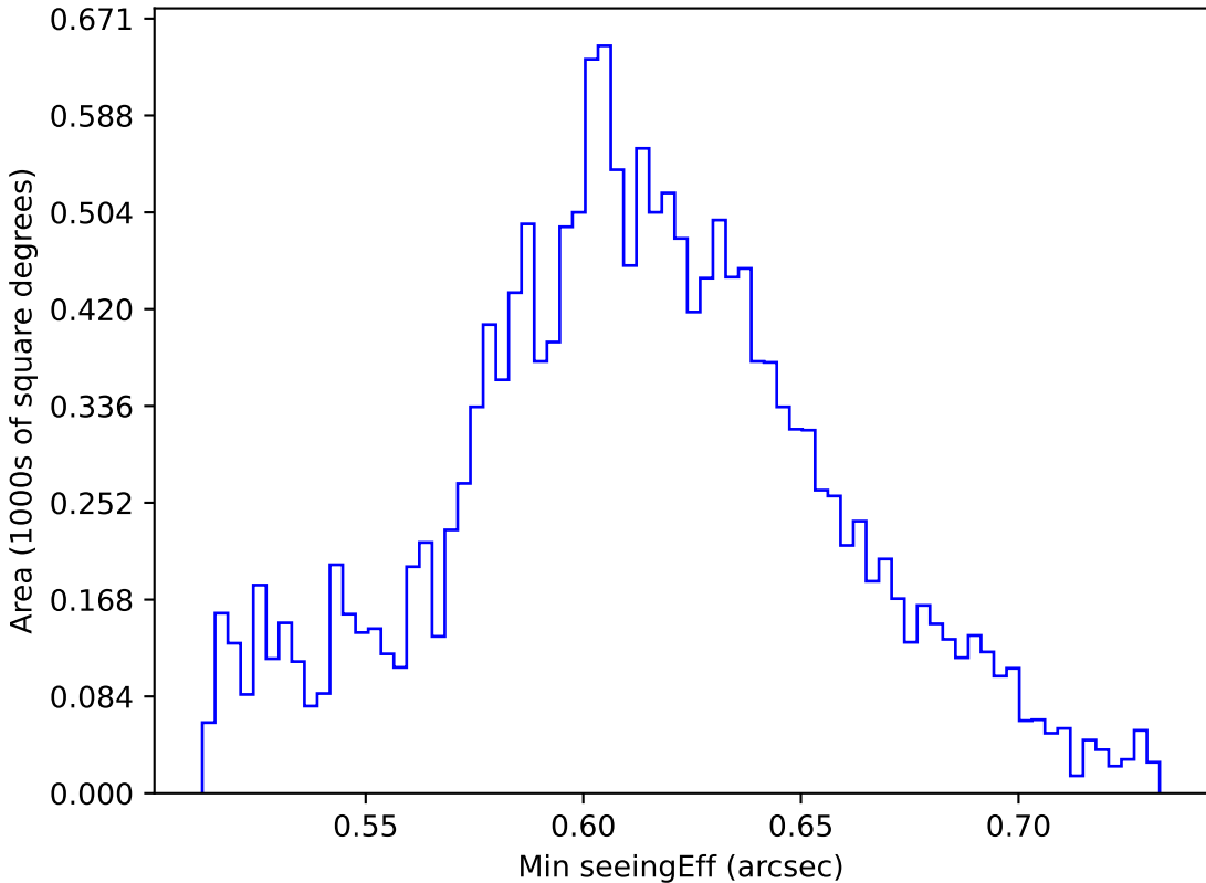
too_elab_r32_d3_giz_v3.4_10yrs WFD z band: Min seeingEff
