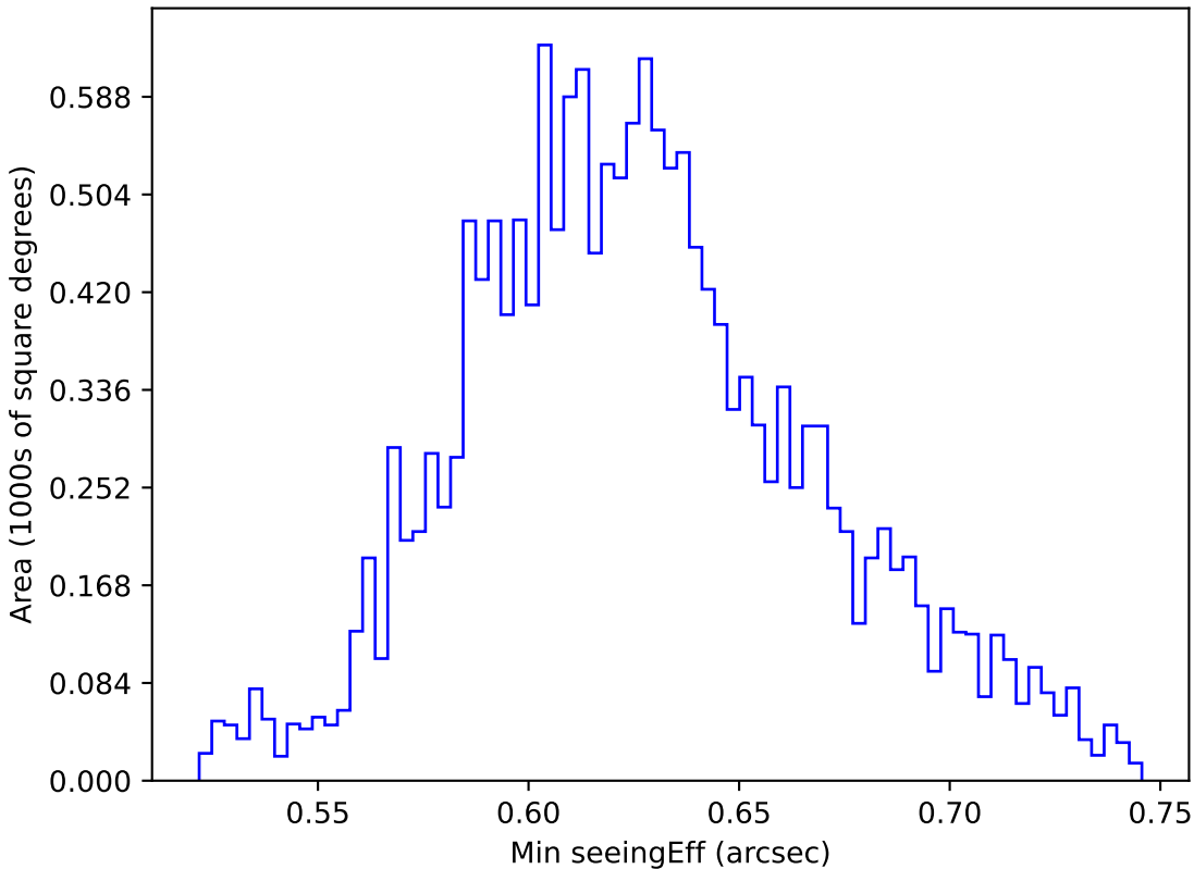
too_elab_r32_d3_giz_v3.4_10yrs WFD y band: Min seeingEff
