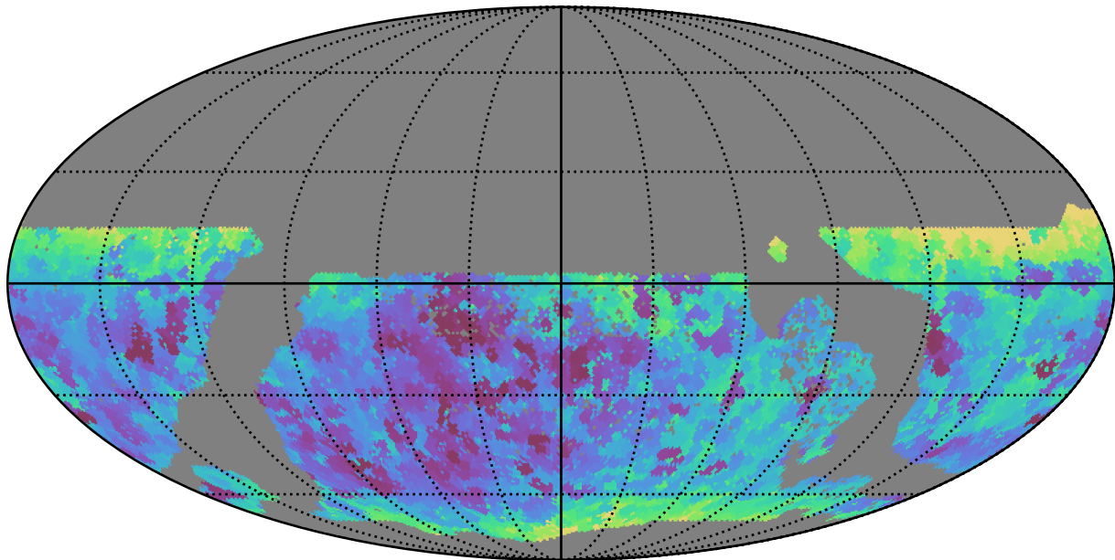
too_elab_r32_d3_giz_v3.4_10yrs WFD all bands: Min seeingEff
