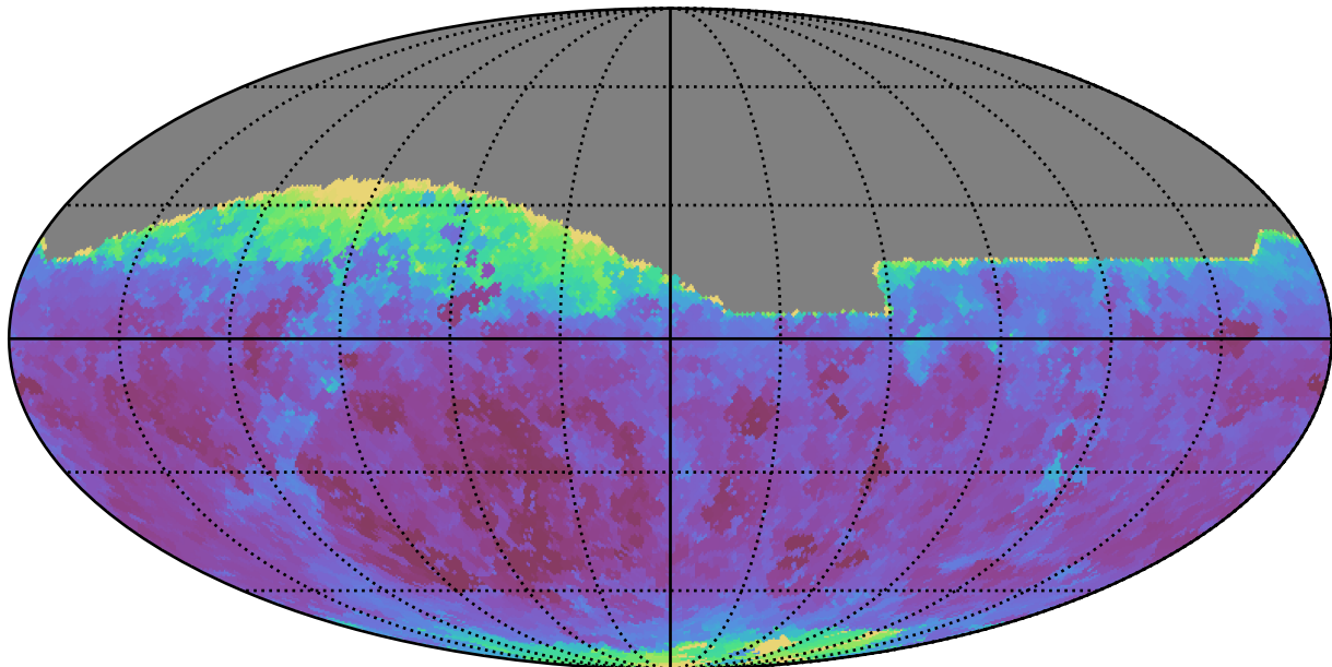
too_elab_r32_d3_giz_v3.4_10yrs All sky z band: Min seeingEff
