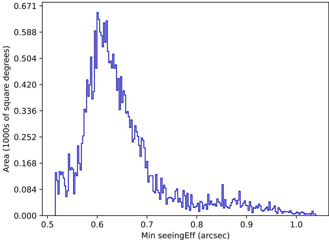
too_elab_r32_d3_giz_v3.4_10yrs All sky z band: Min seeingEff
