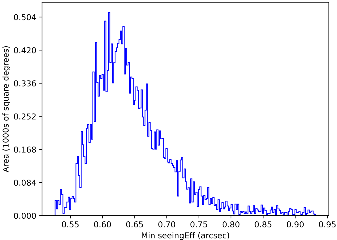
too_elab_r32_d3_giz_v3.4_10yrs All sky y band: Min seeingEff
