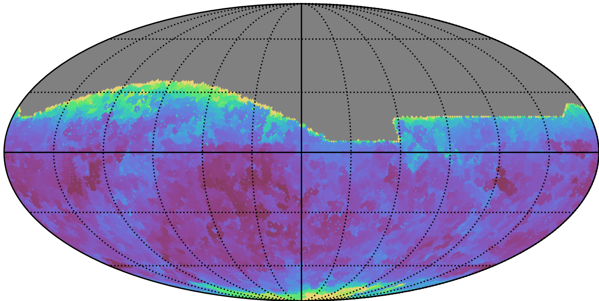
too_elab_r32_d3_giz_v3.4_10yrs All sky i band: Min seeingEff
