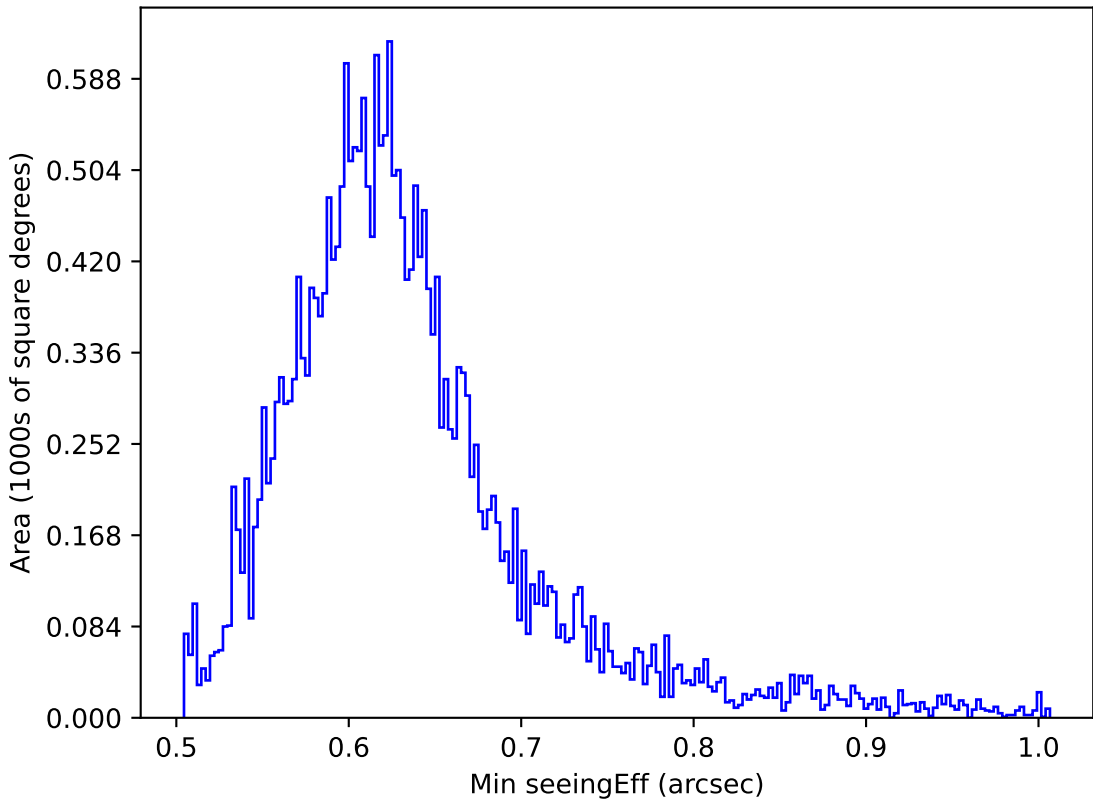
too_elab_r32_d3_giz_v3.4_10yrs All sky i band: Min seeingEff
