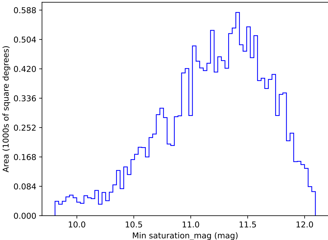
too_elab_r32_d3_giz_v3.4_10yrs WFD y band: Min saturation_mag
