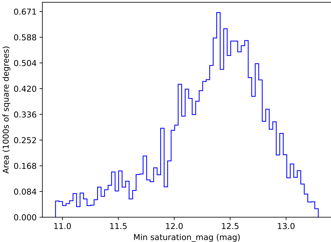
too_elab_r32_d3_giz_v3.4_10yrs WFD i band: Min saturation_mag
