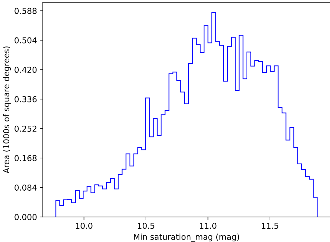
too_elab_r32_d3_giz_v3.4_10yrs WFD all bands: Min saturation_mag
