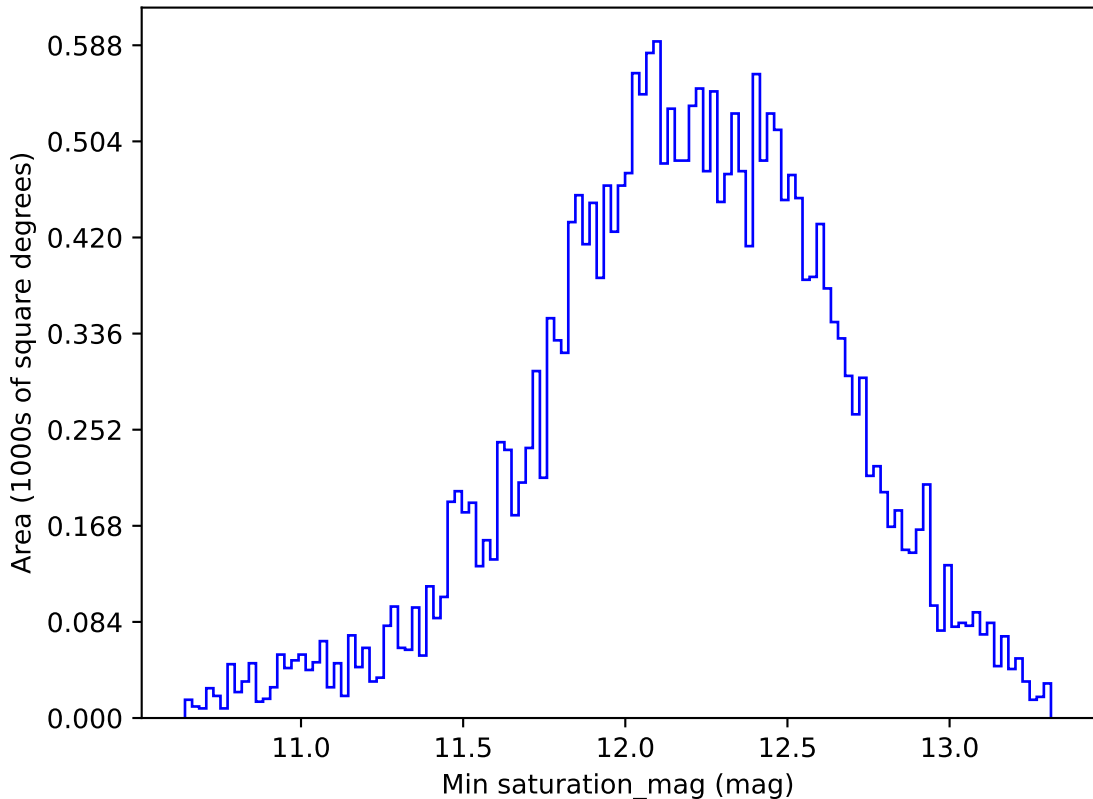
too_elab_r32_d3_giz_v3.4_10yrs All sky z band: Min saturation_mag
