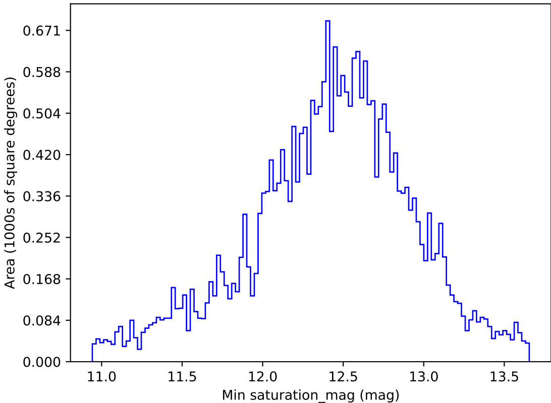
too_elab_r32_d3_giz_v3.4_10yrs All sky i band: Min saturation_mag
