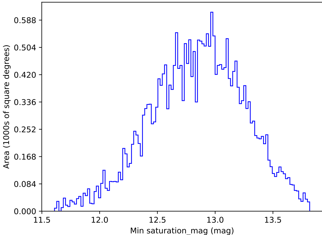
too_elab_r32_d3_giz_v3.4_10yrs All sky g band: Min saturation_mag
