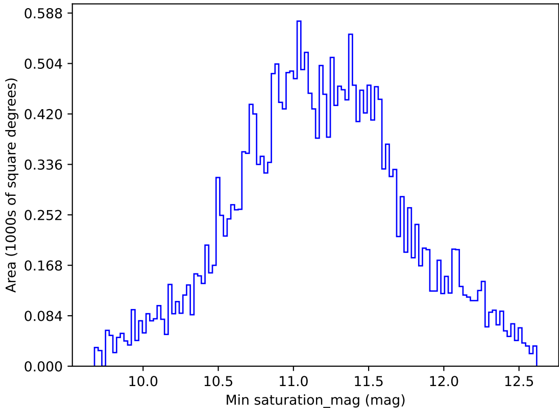
too_elab_r32_d3_giz_v3.4_10yrs All sky all bands: Min saturation_mag
