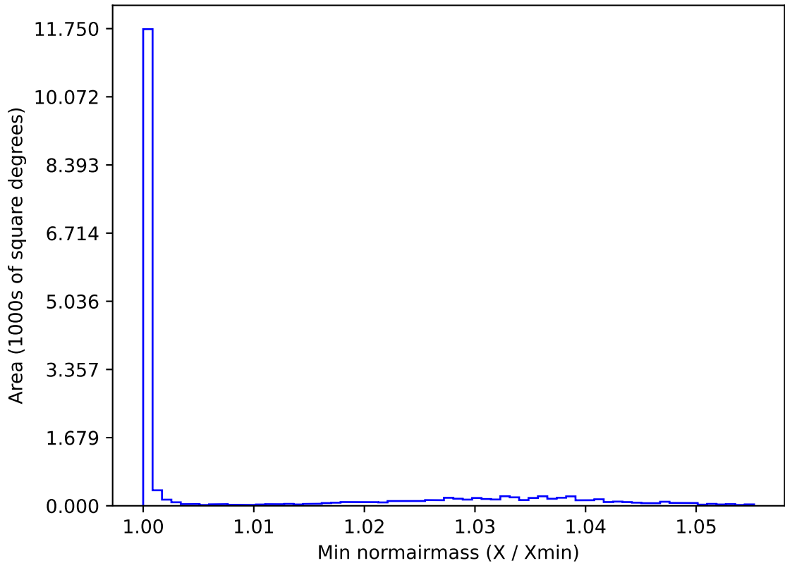
too_elab_r32_d3_giz_v3.4_10yrs WFD u band: Min normairmass
