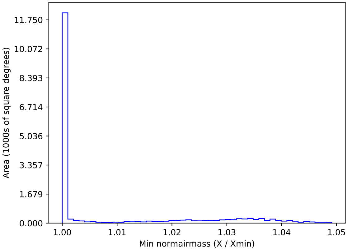
too_elab_r32_d3_giz_v3.4_10yrs WFD g band: Min normairmass
