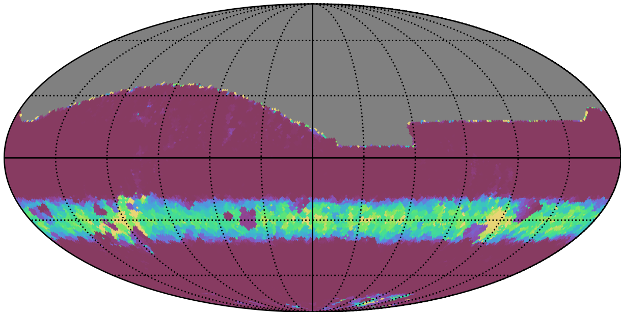
too_elab_r32_d3_giz_v3.4_10yrs All sky z band: Min normairmass
