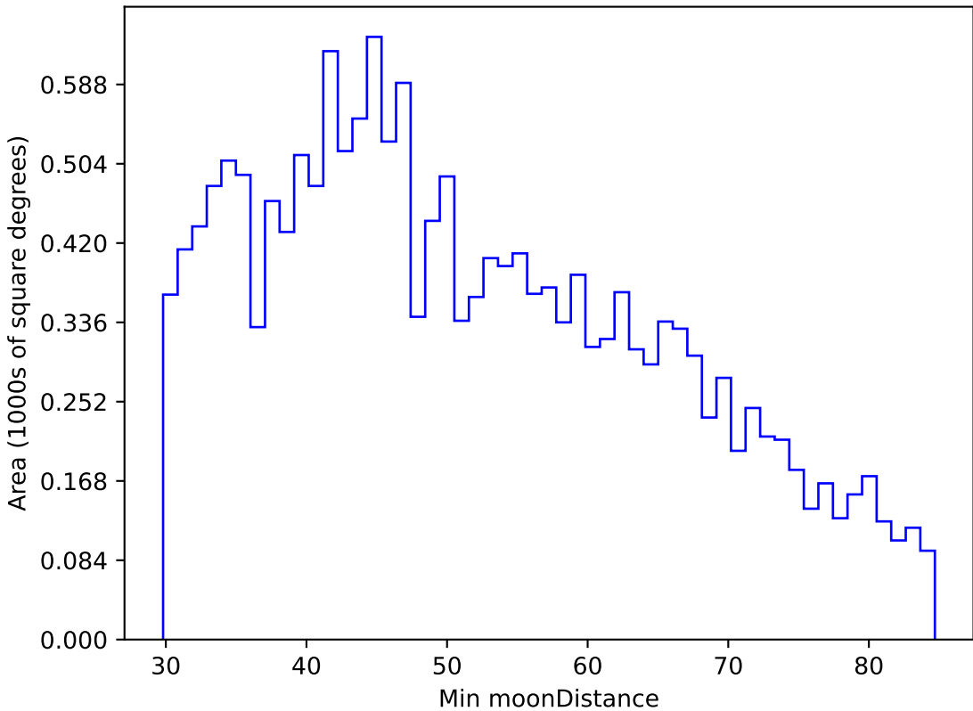
too_elab_r32_d3_giz_v3.4_10yrs WFD u band: Min moonDistance
