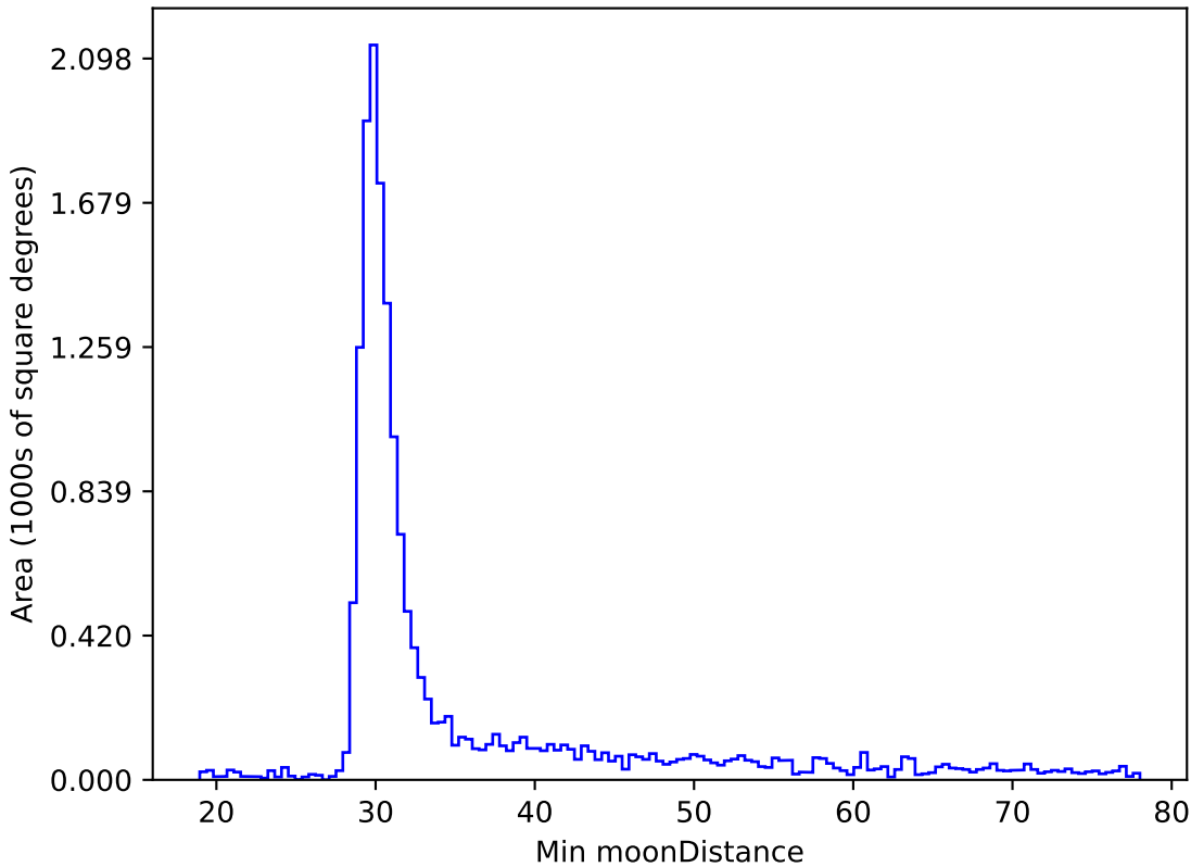
too_elab_r32_d3_giz_v3.4_10yrs WFD i band: Min moonDistance
