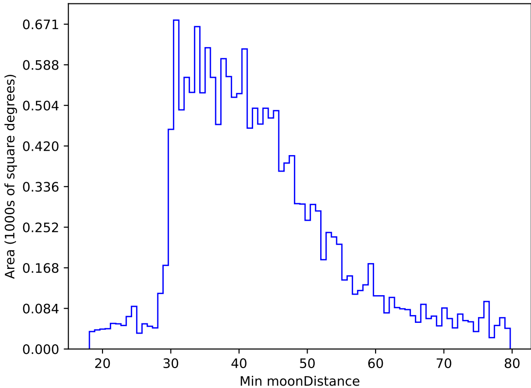
too_elab_r32_d3_giz_v3.4_10yrs WFD g band: Min moonDistance
