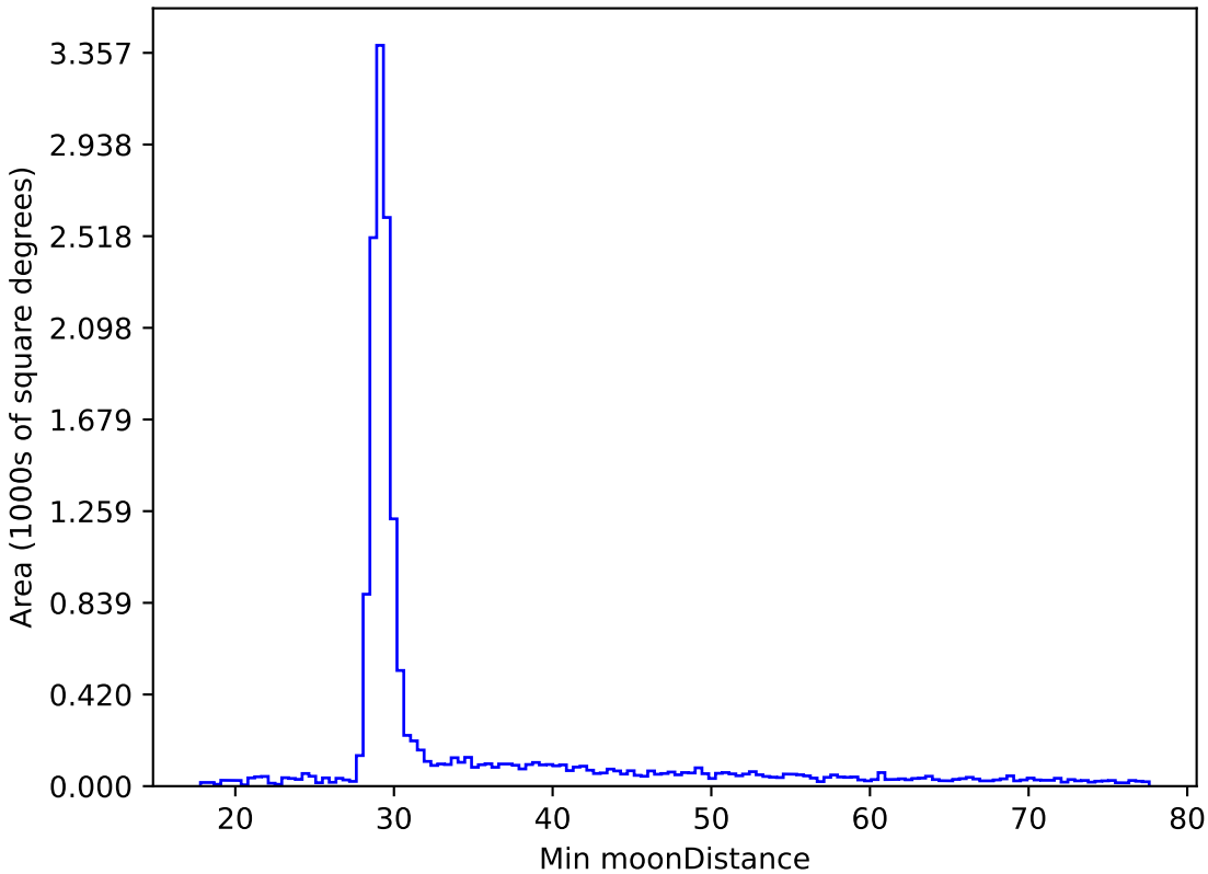
too_elab_r32_d3_giz_v3.4_10yrs WFD all bands: Min moonDistance
