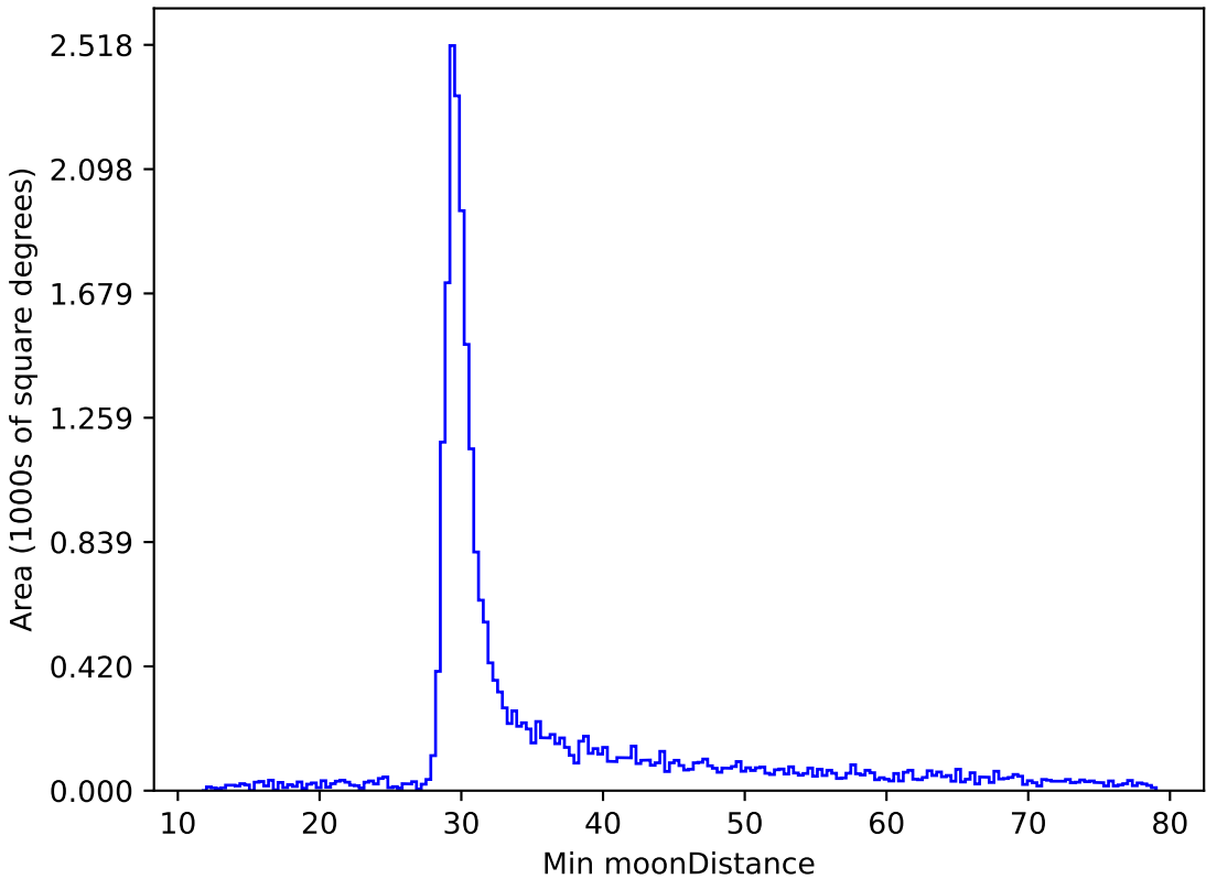
too_elab_r32_d3_giz_v3.4_10yrs All sky z band: Min moonDistance
